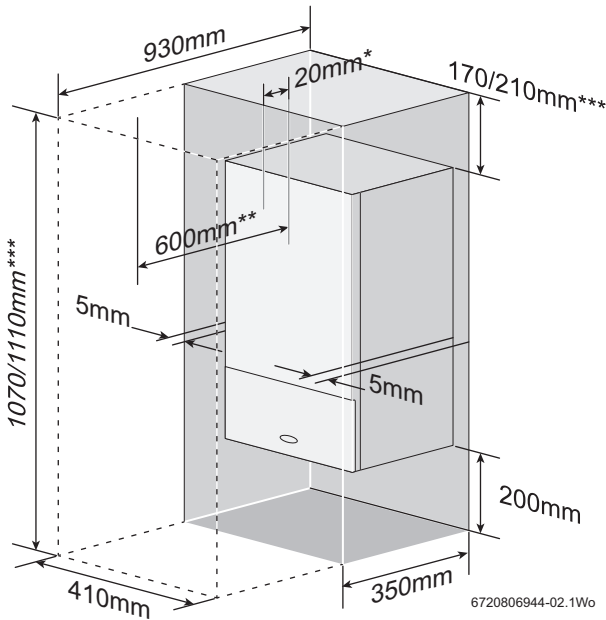
Fig. 15 Unventilated compartment
