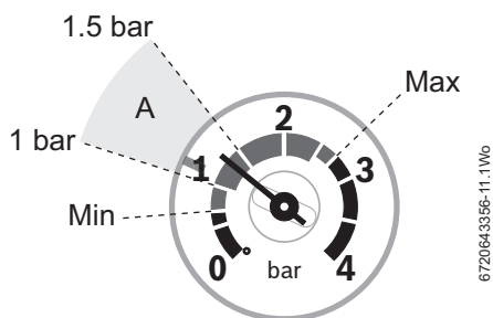
Fig. 2 Optimum system pressure when your boiler is cold (area A)
