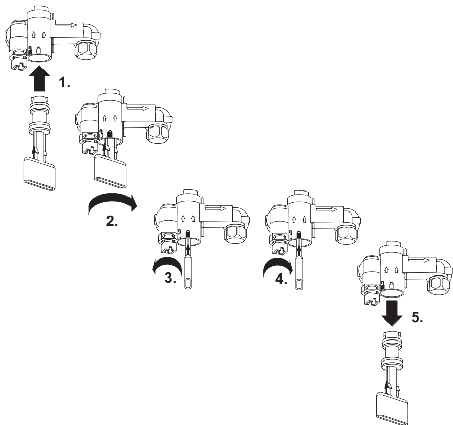
Fig. 3 Inserting the filling key
